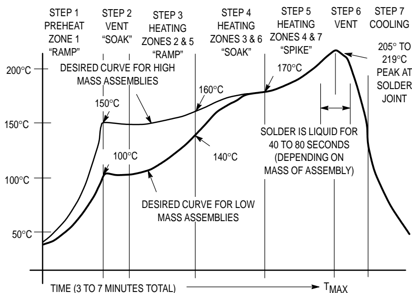
Figure 6. Typical Solder Heating Profile
