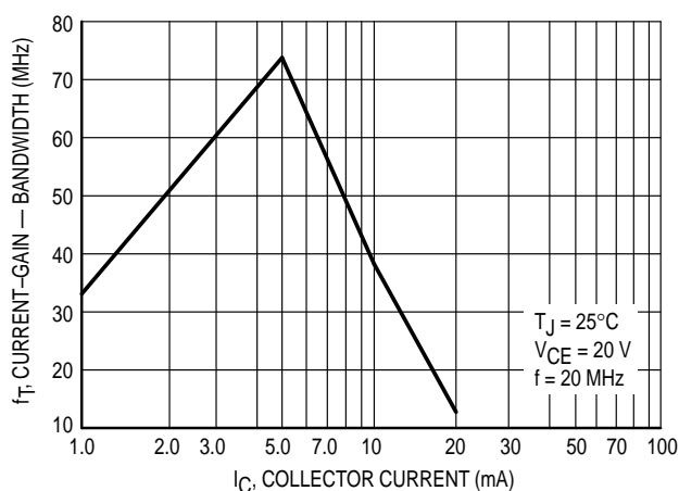
Figure 3. Current-Gain - Bandwidth
