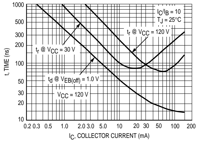
Figure 8. Turn-On Time
