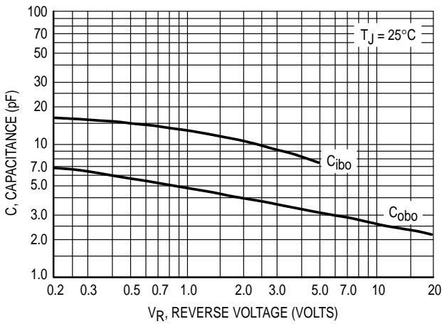
Figure 7. Capacitances
