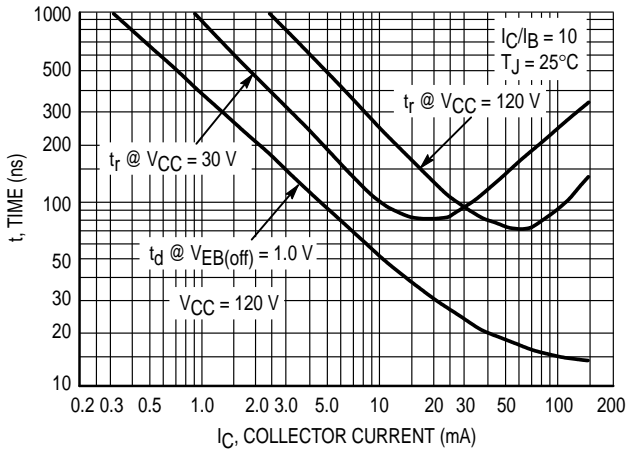
Figure 8. Turn-On Time
