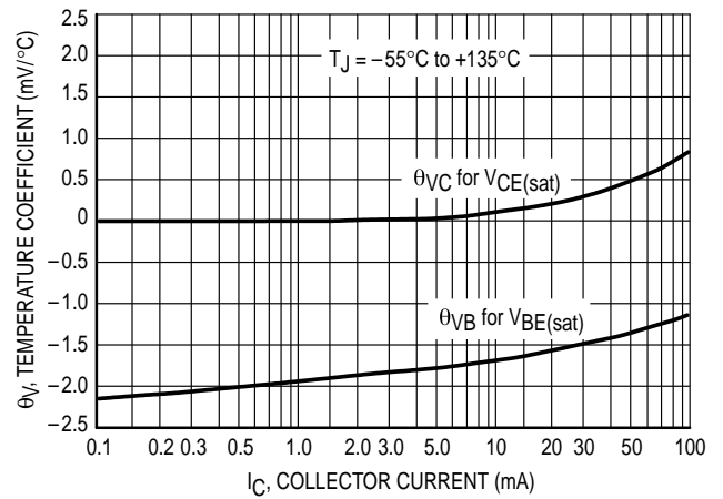
Figure 5. Temperature Coefficients
