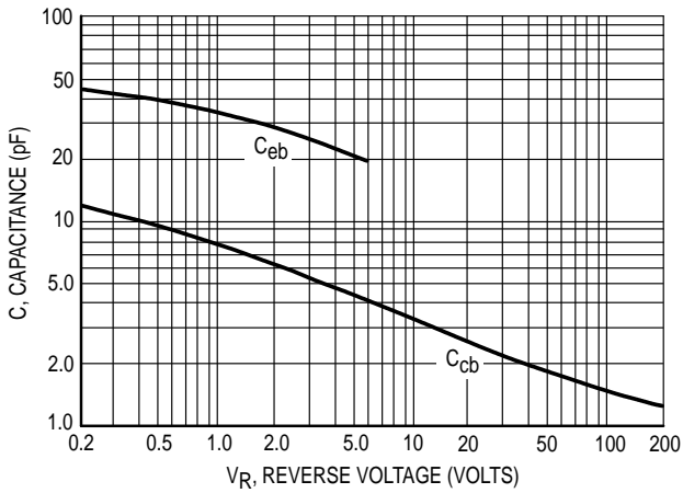
Figure 2. Capacitances
