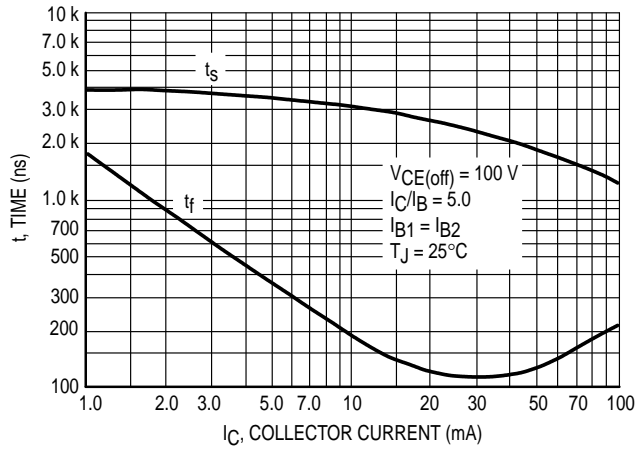
Figure 7. Turn-Off Time
