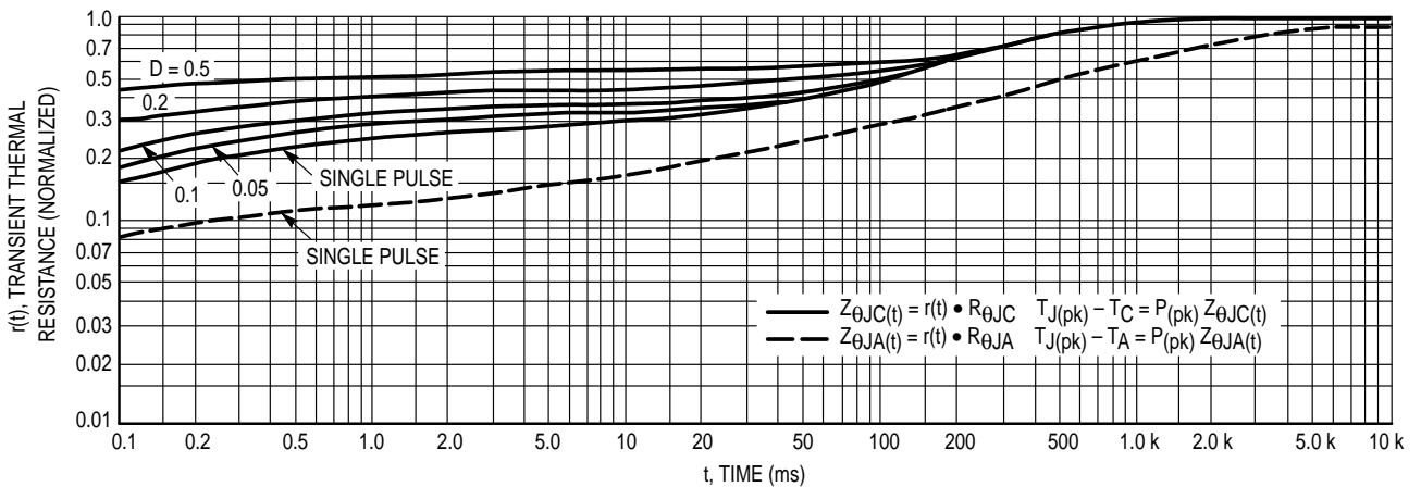
Figure 9. Thermal Response
