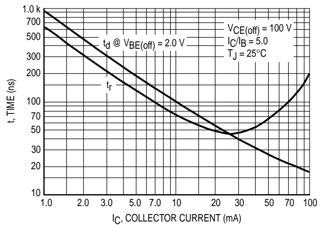
Figure 6. Turn-On Time
