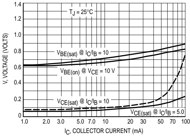
Figure 3. "On" Voltages
