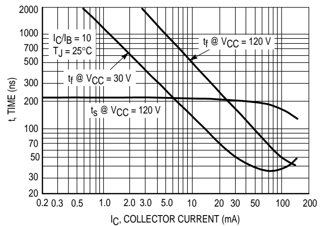
Figure 9. Turn-Off Time
