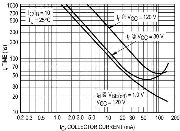
Figure 8. Turn-On Time
