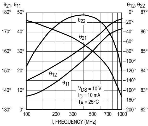
Figure 8. Common-Gate Y Parameter Phase-Angle versus Frequency
