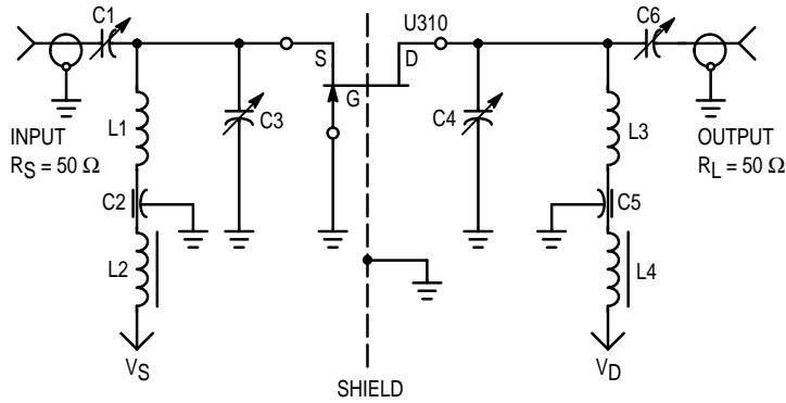
Figure 12. 450 MHz IMD Evaluation Amplifier
