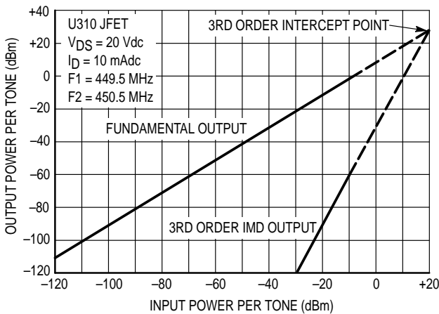
Figure 13. Two Tone 3rd Order Intercept Point
