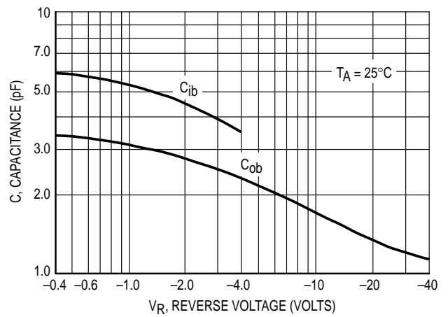
Figure 4. Capacitance
