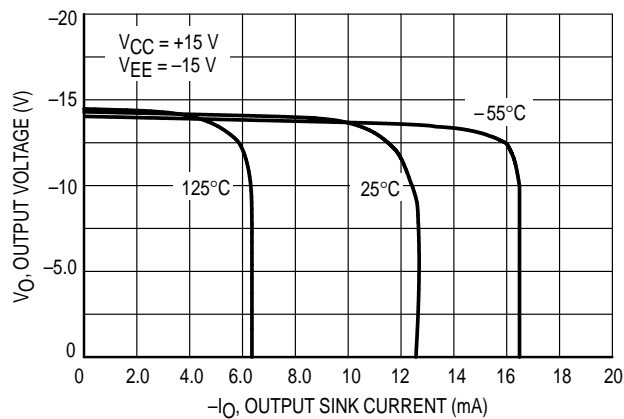
Figure 8. Output Voltage versus Output Sink Current
