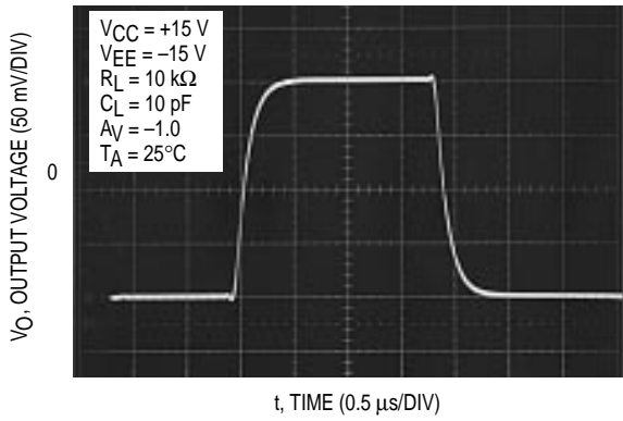
Figure 23. Inverting
