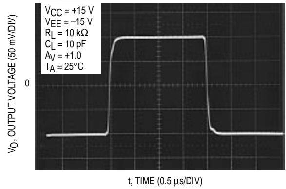
Figure 24. Noninverting
