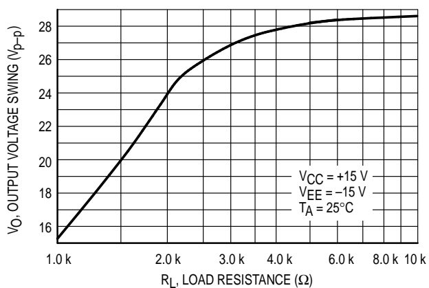
Figure 10. Output Voltage Swing versus Load Resistance
