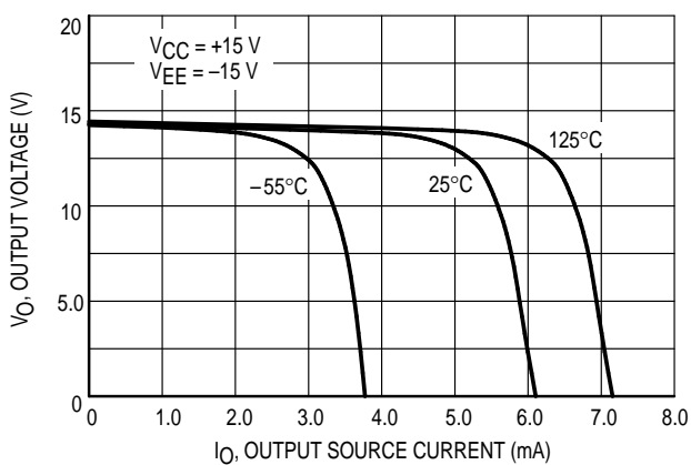
Figure 7. Output Voltage versus Output Source Current
