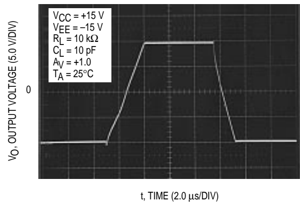
Figure 26. Noninverting
