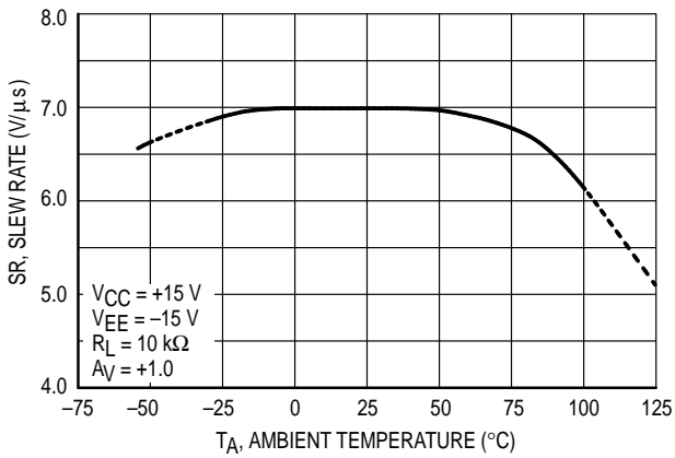
Figure 13. Slew Rate versus Temperature
