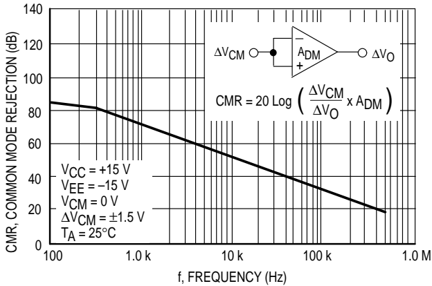
Figure 17. Common Mode Rejection versus Frequency
