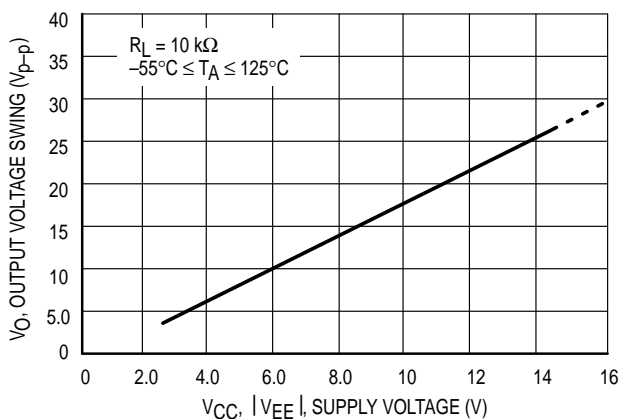
Figure 9. Output Voltage Swing versus Supply Voltage
