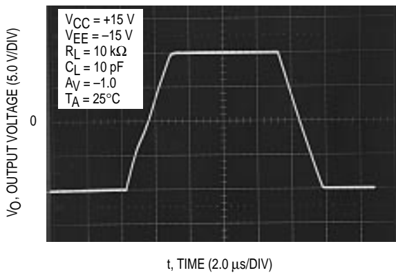
Figure 25. Inverting
