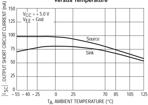
Figure 14. Output Short Circuit Current versus Temperature
