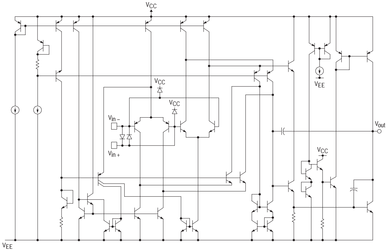
Figure 1. Circuit Schematic (Each Amplifier)
