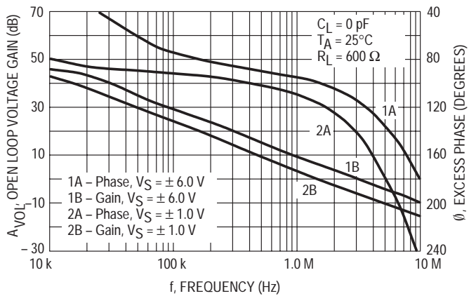
Figure 19. Voltage Gain and Phase versus Frequency
