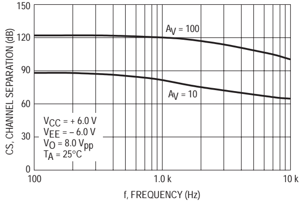
Figure 23. Channel Separation versus Frequency
