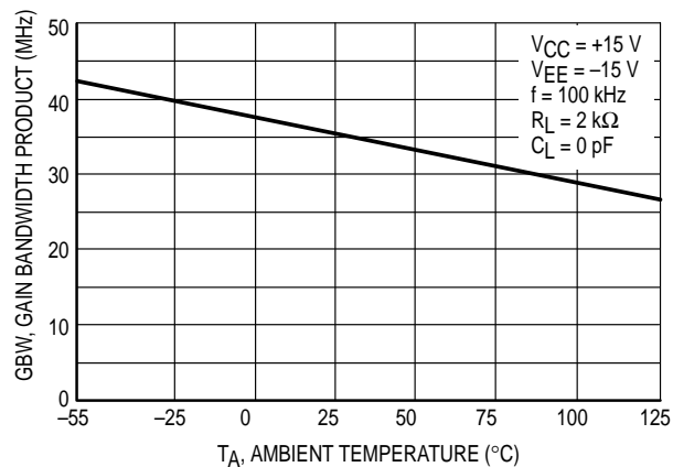
Figure 17. Gain Bandwidth Product versus Temperature
