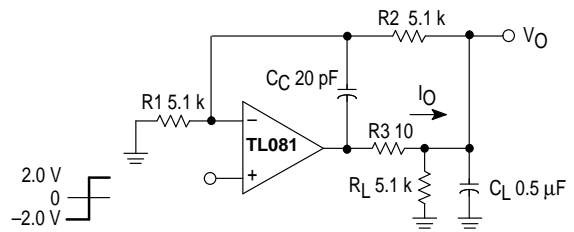
Figure 17. Isolating Large Capacitive Loads
