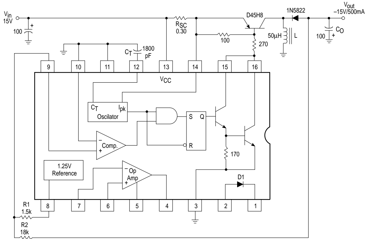
Figure 7. Inverting Converter
