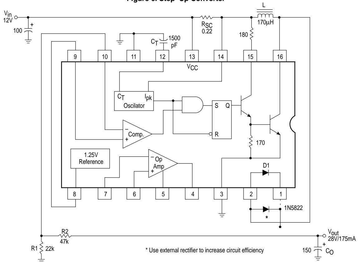
Figure 6. Step-Up Converter
