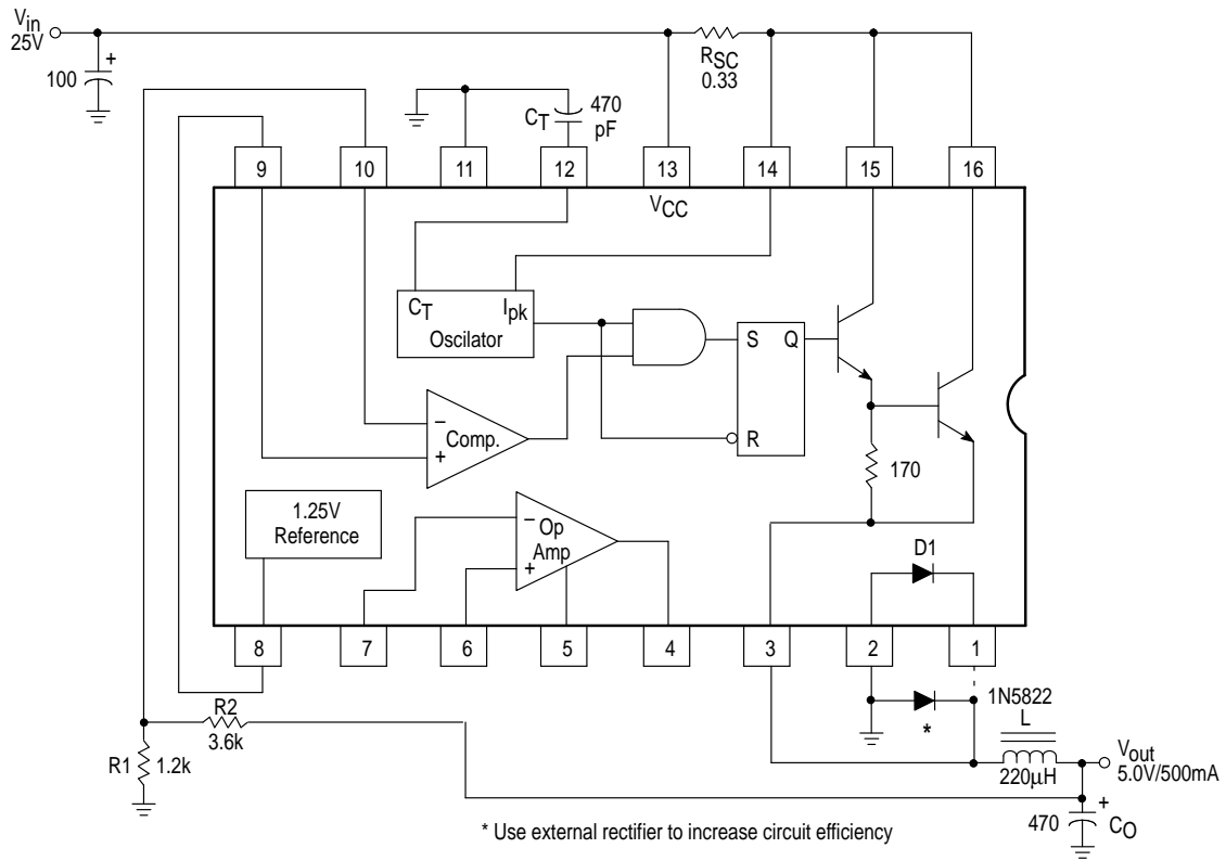
Figure 5. Step-Down Converter
