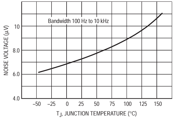
Figure 14. Output Noise
