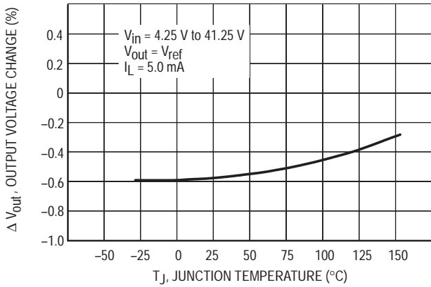
Figure 13. Line Regulation
