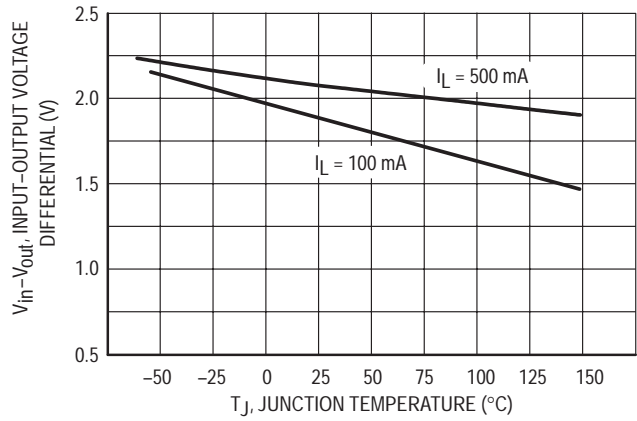
Figure 8. Dropout Voltage
