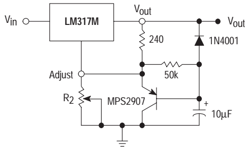
Figure 21. Slow Turn-On Regulator
