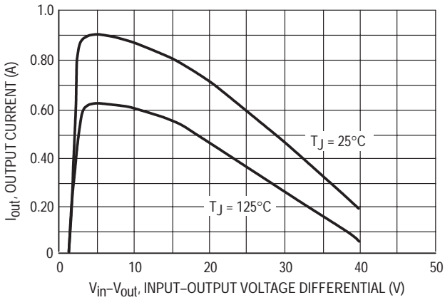
Figure 7. Current Limit
