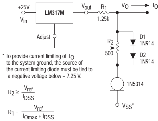
Figure 19. Adjustable Current Limiter
