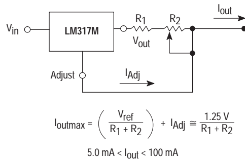
Figure 22. Current Regulator
