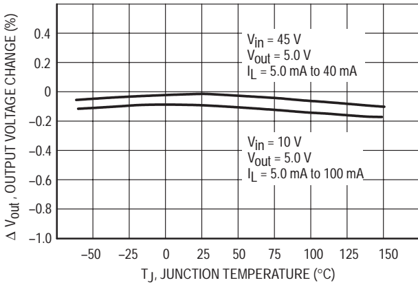
Figure 5. Load Regulation
