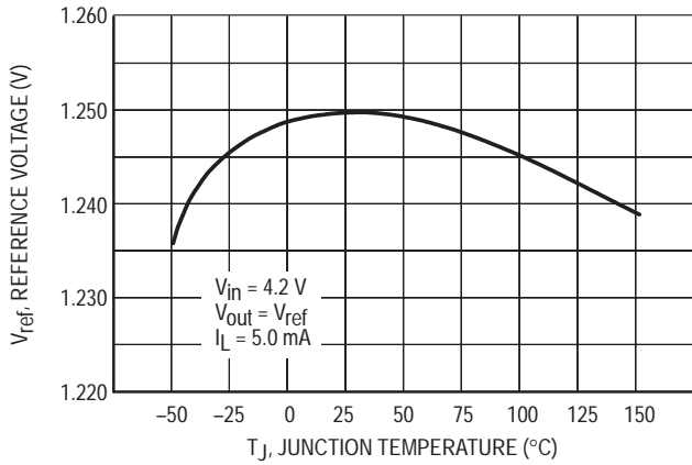
Figure 11. Temperature Stability
