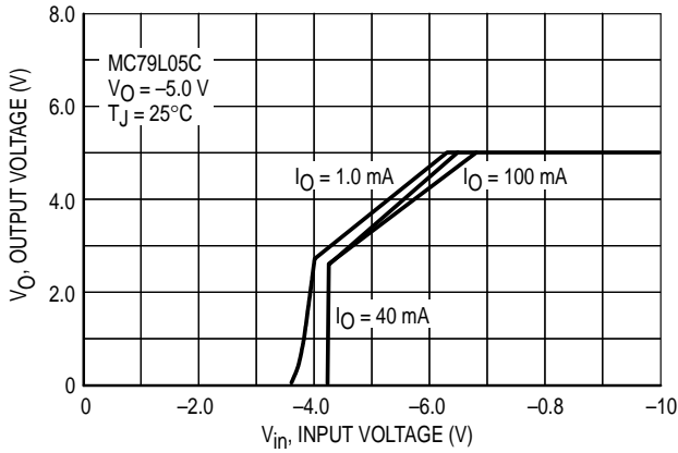
Figure 3. Dropout Characteristics
