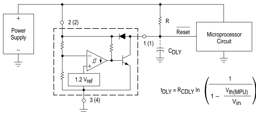
Figure 13. Low Voltage Microprocessor Reset
