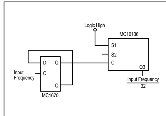
FIGURE 2 — 300 MHz PRESCALER
