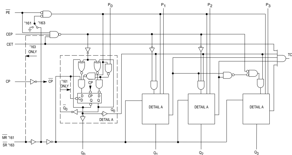
LOGIC DIAGRAM
