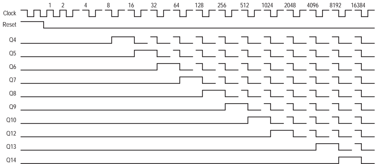
Figure 6. Timing Diagram
