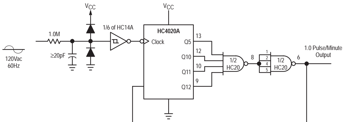
Figure 7. Time-Base Generator
