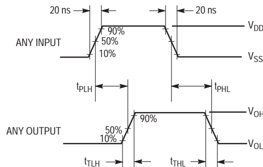
Figure 1. Switching Time Waveforms
