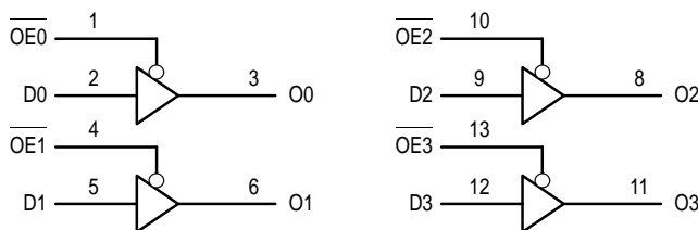
Figure 2. Logic Diagram
