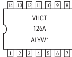
14-LEAD TSSOP DT SUFFIX CASE 948G
