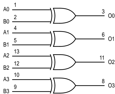
Figure 2. Logic Diagram
