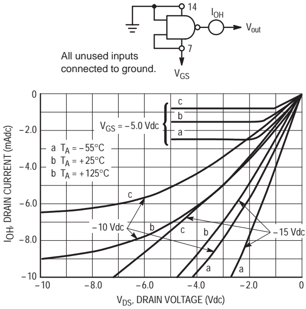
Figure 3. Typical Output Source Characteristics Test Circuit
