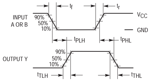
Figure 1. Switching Waveforms
