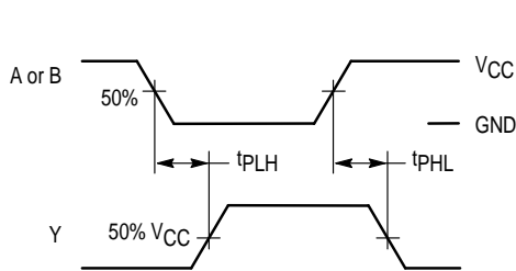
Figure 1. Switching Waveforms
