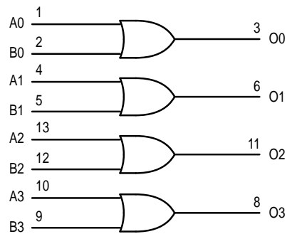
Figure 2. Logic Diagram
