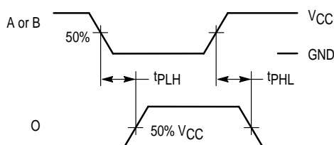
Figure 3. Switching Waveforms
