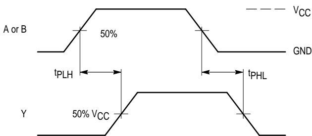
Figure 1. Switching Waveforms
