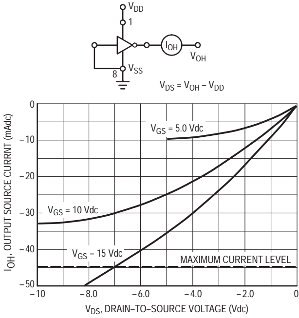
Figure 2. Typical Output Source Characteristics
