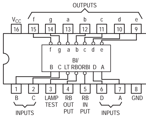
SN74LS247 (TOP VIEW)
