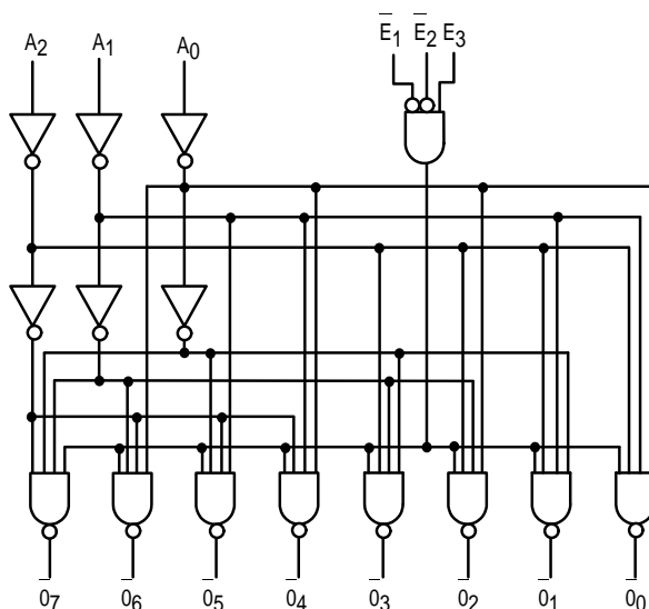
LOGIC DIAGRAM
