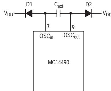
Figure 2. Discharge Protection During Power Down
