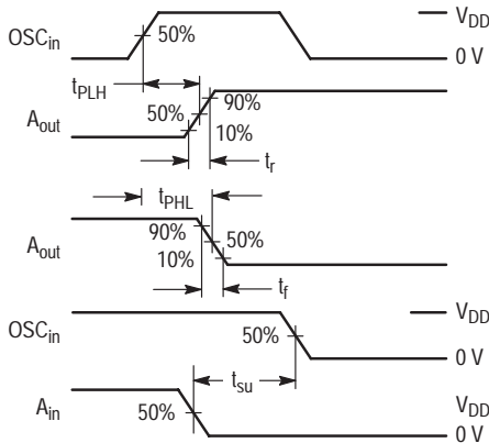
Figure 1. Switching Waveforms
