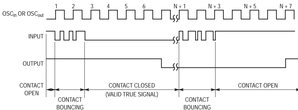
Figure 3. Timing Diagram
