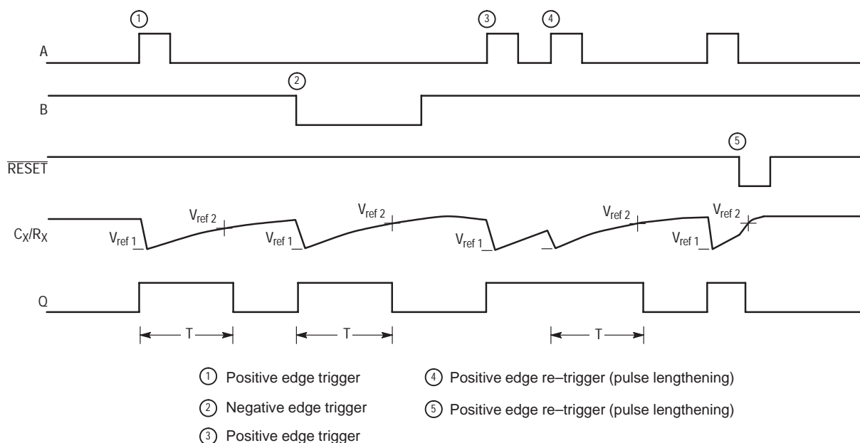
Figure 10. Timing Operation
