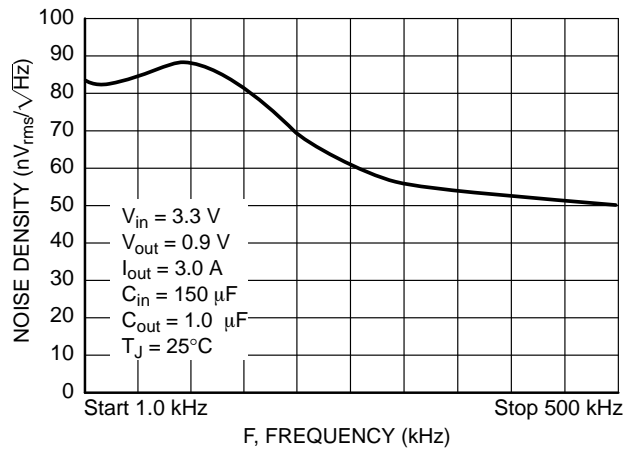
Figure 10. Noise Density vs. Frequency
