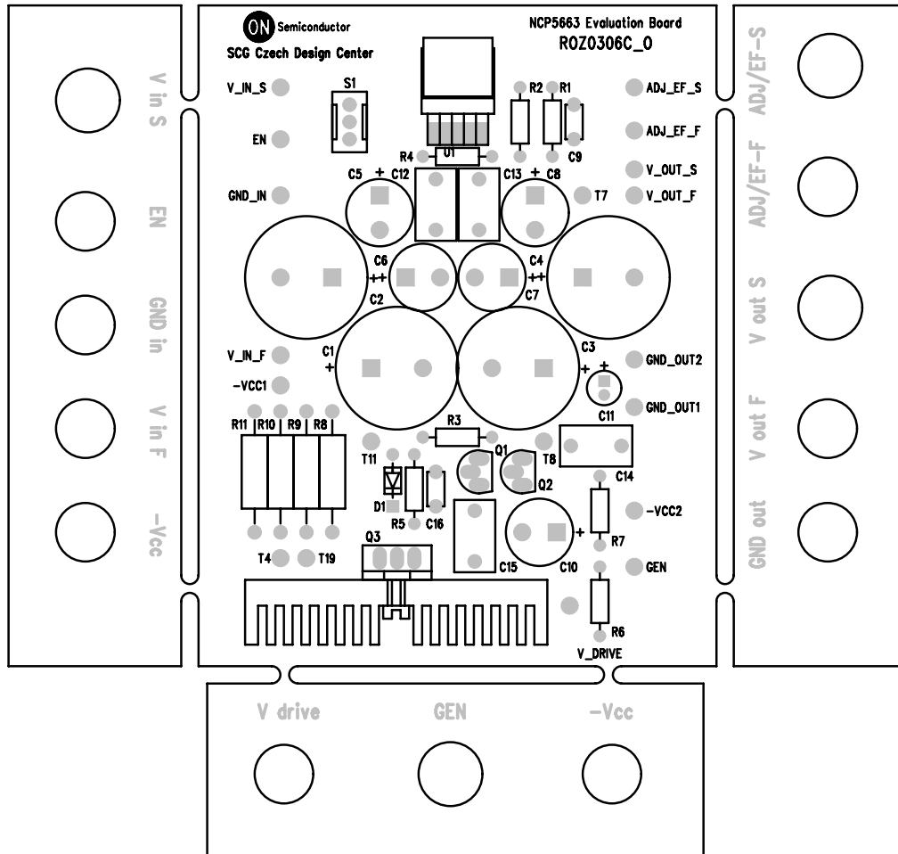
Figure 17. Test Board used for Evaluation
