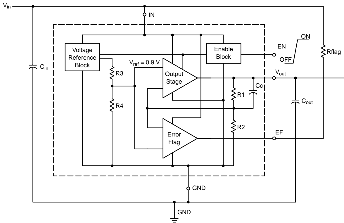
Figure 2. Typical Schematic, Fixed Output Version
