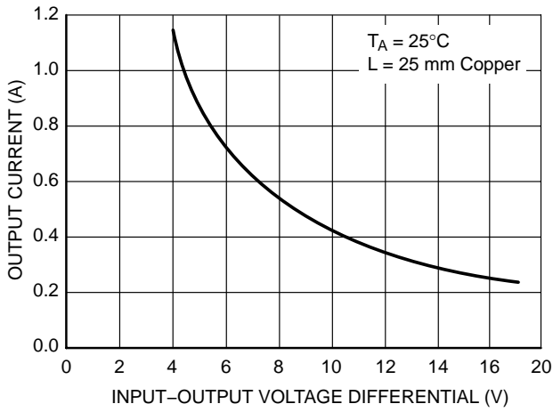
Figure 7. Output Current vs. Input-Output Voltage Differential
