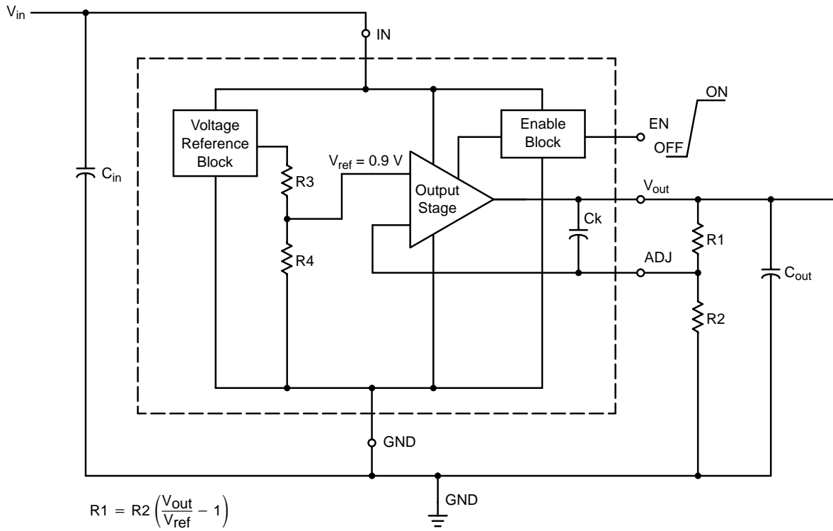
Figure 1. Typical Schematic, Adjustable Output Version
