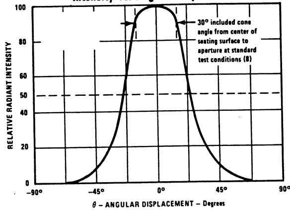
OP290/OP291/OP292 Relative Radiant Intensity vs. Angular Displacement
