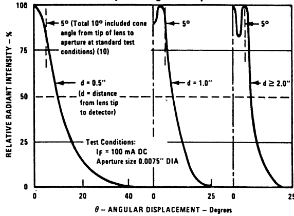
OP295/OP296/OP297 Relative Radiant Intensity vs. Angular Displacement
