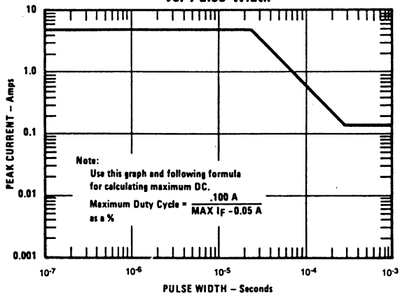
Maximum Peak Pulse Current vs. Pulse Width
