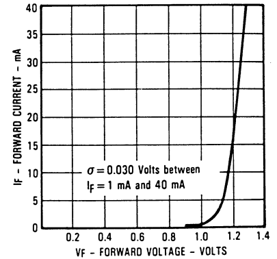
Forward Current vs Forward Voltage Input Diode
