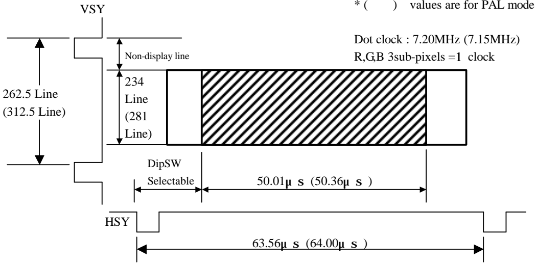
Fig6-2 4:3 mode (Center/Right/Left)
