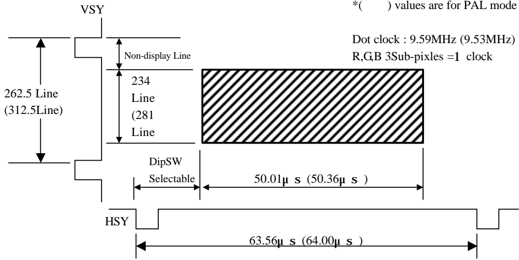
Fig.6-1 Full/Wide/Zoom1,2 mode
