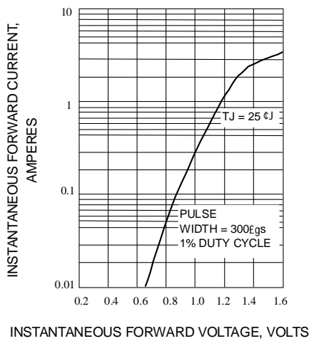
INSTANTANEOUS FORWARD VOLTAGE, VOLTS
