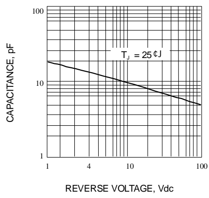
Fig. 4-TYPICAL JUNCTION CAPACITANCE
