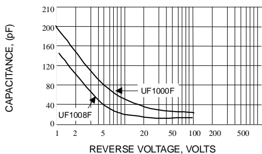
Fig. 4-TYPICAL JUNCTION CAPACITANCE
