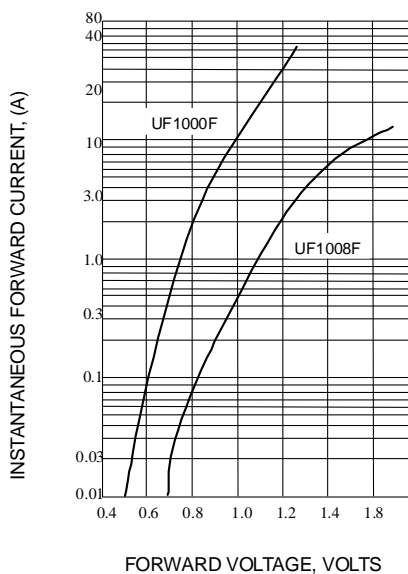
Fig. 5-TYPICAL FORWARD CHARACTERISTICS
