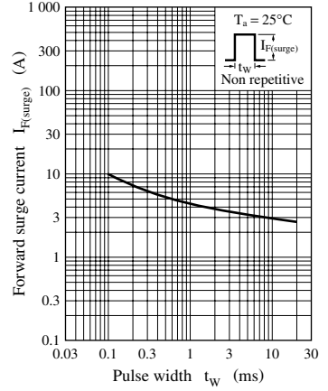
I_{F(\text{surge})} - t_w
