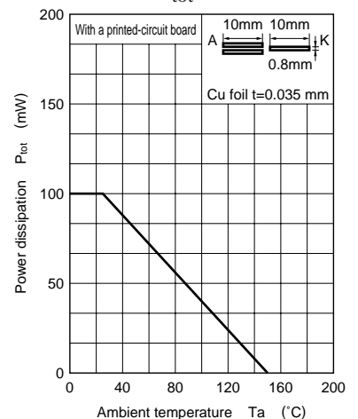
P_{tot} - T_a
