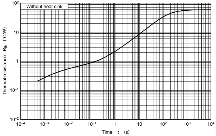
R_{th(t)} - t
