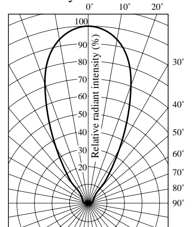
Directivity characteristics
