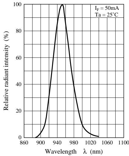
Spectral characteristics
