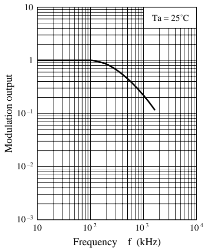
Frequency characteristics
