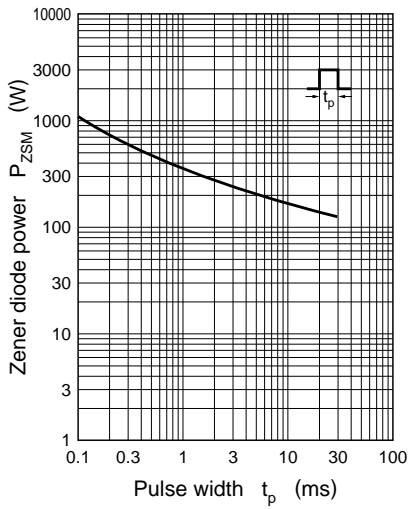
P_{ZSM} - t_p
