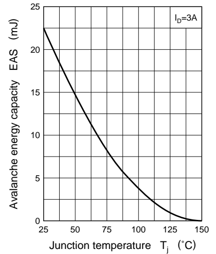
EAS — T_j
