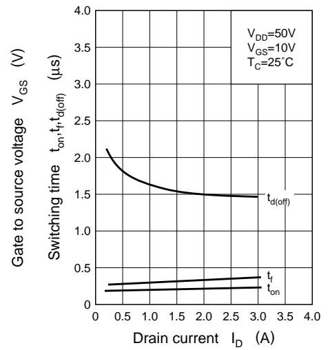
t_{on}, t_f, t_{d(off)} - I_D
