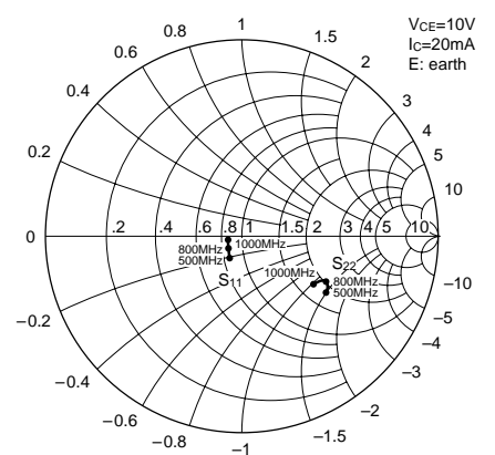
S_{11}, S_{22}
