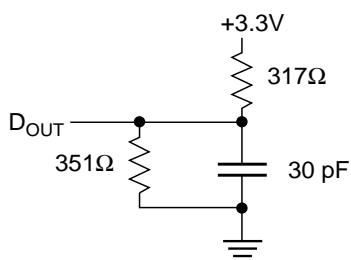
Figure 1. Output Load Equivalent
