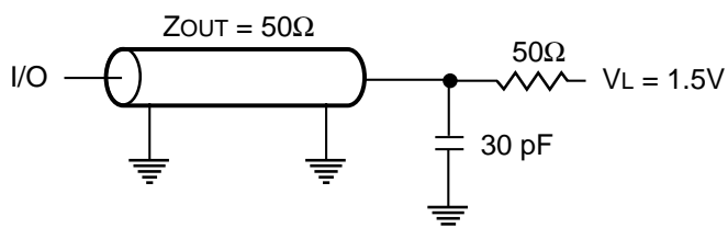
Figure 1. Output Load
