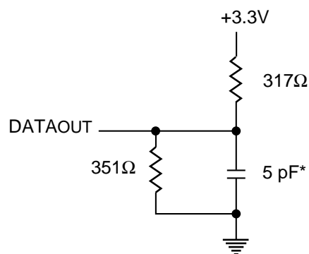
Figure 2. Output Load
