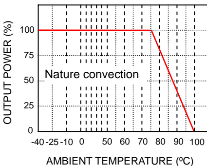
Derating Curve with Heat-Sink
