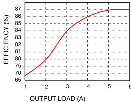
Efficiency VS Output load
